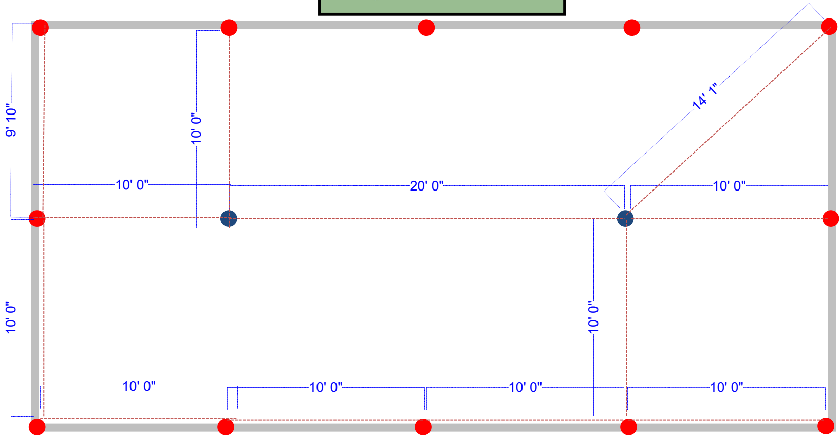
20' x 40' Pole Tent - Pole placement
