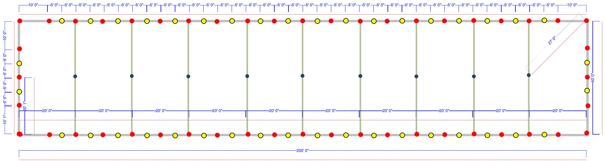
40' x 200' Pole Tent Standard & Wind - Pole Placements
