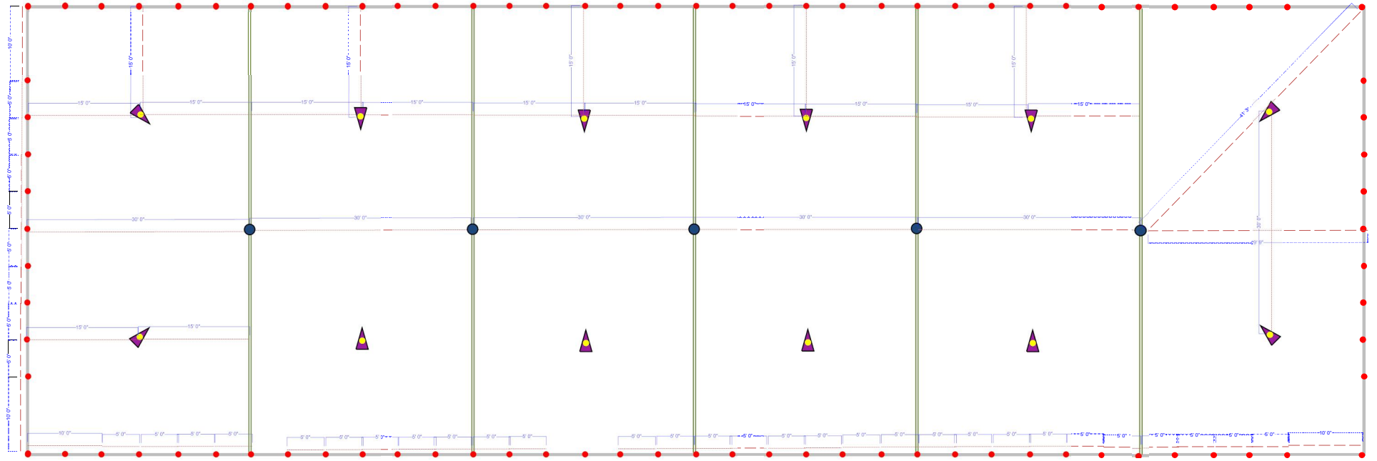
60' x 180' Pole Tent - Pole Placements
