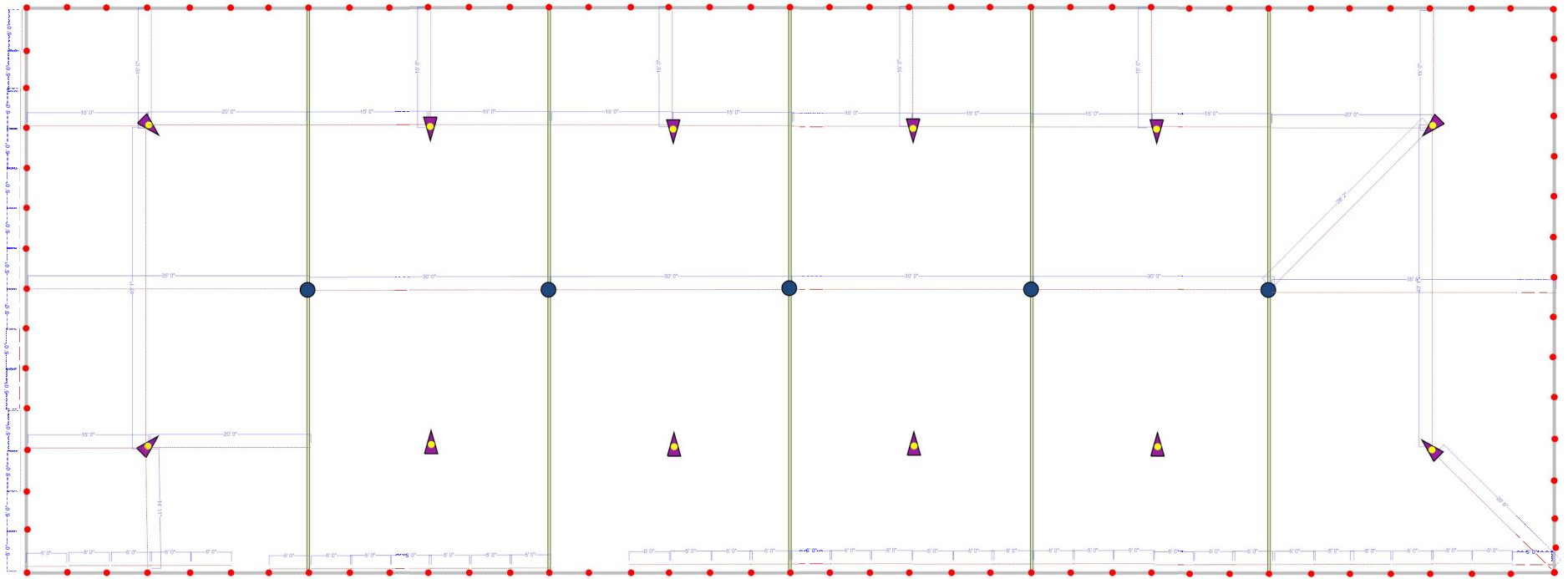
70' x 190' Pole Tent - Pole Placements
