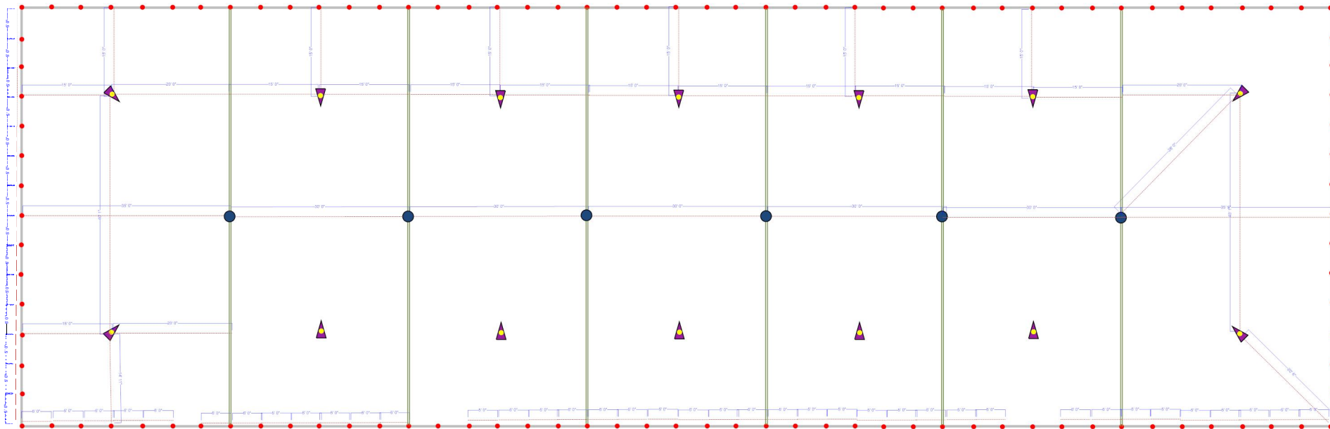
70' x 220' Pole Tent - Pole Placements
